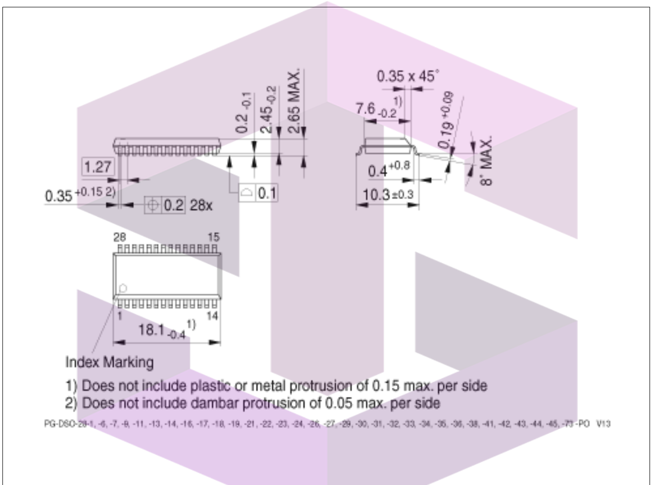
Figure 19 PG-DSO-28
