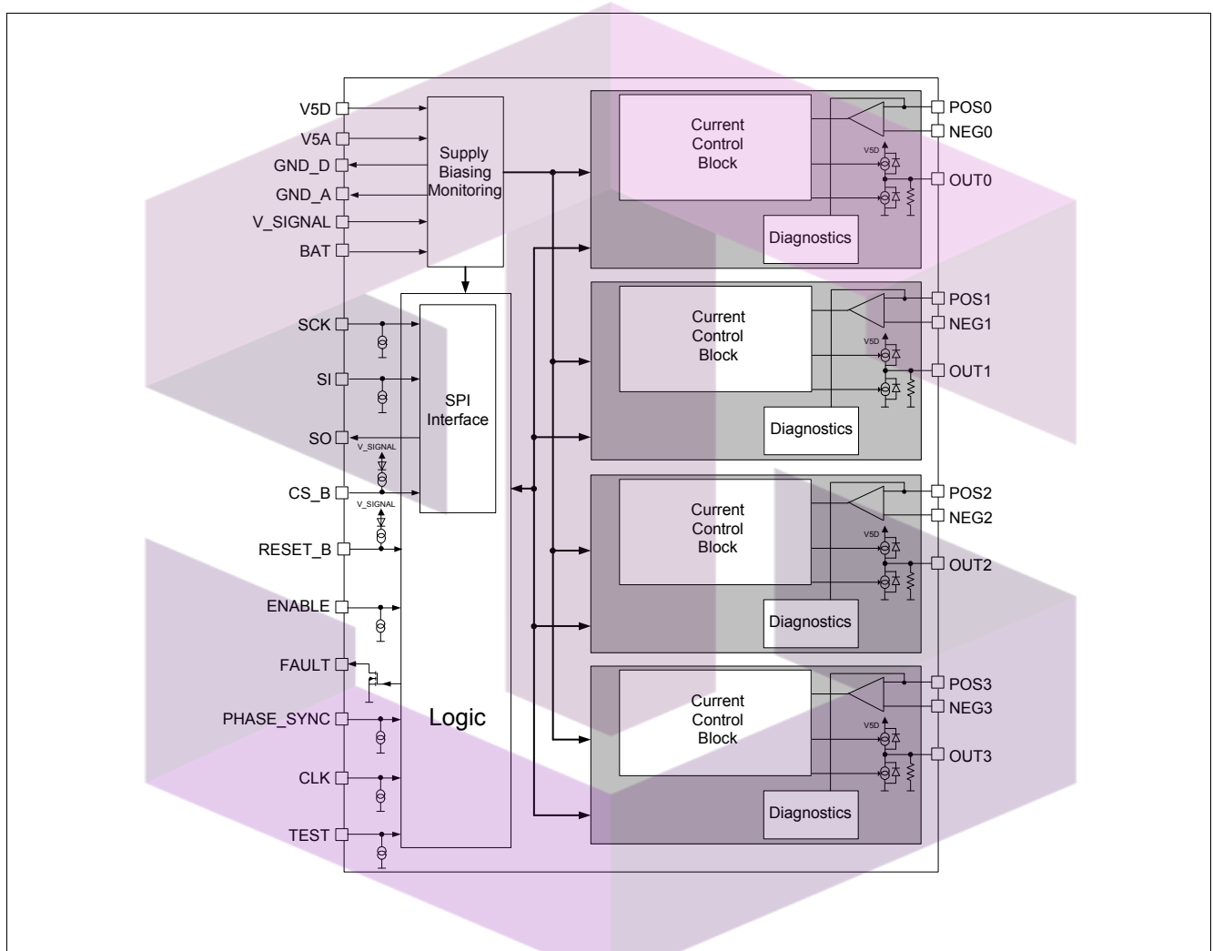
Figure 7 Block Diagram
